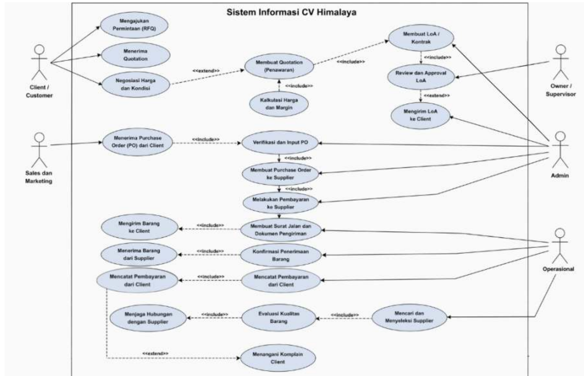
Gambar Use Case Diagram
